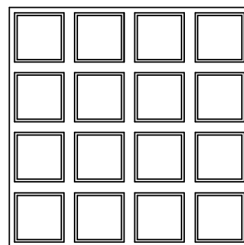
16 Furos (43x39,5x7,5)
